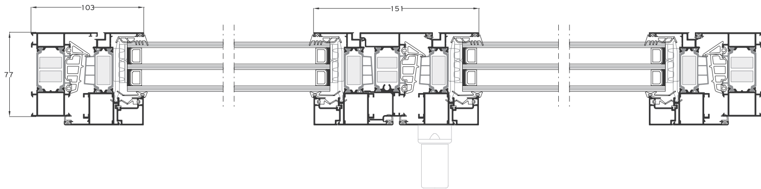
2 Sashes Narrow Adjoining Profile
