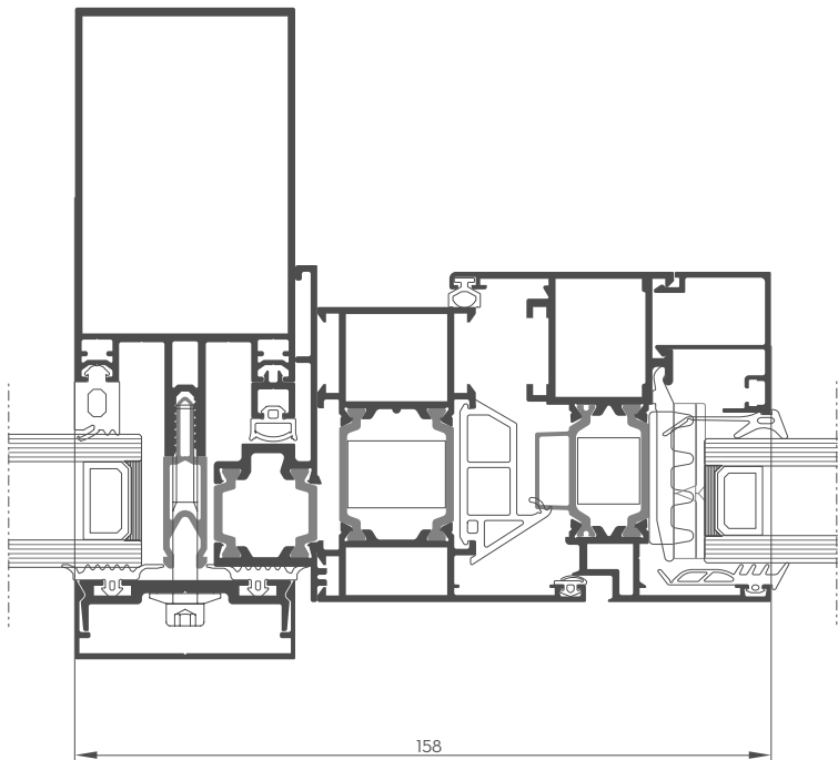
Standard Tilt & Turn Window
